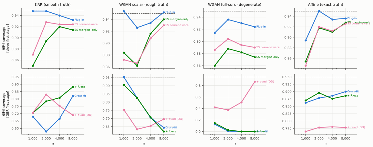
Figure 1: Empirical 95% coverage by sample size, DGP (columns), and first-stage family (rows). Dashed line: nominal 0.95.
